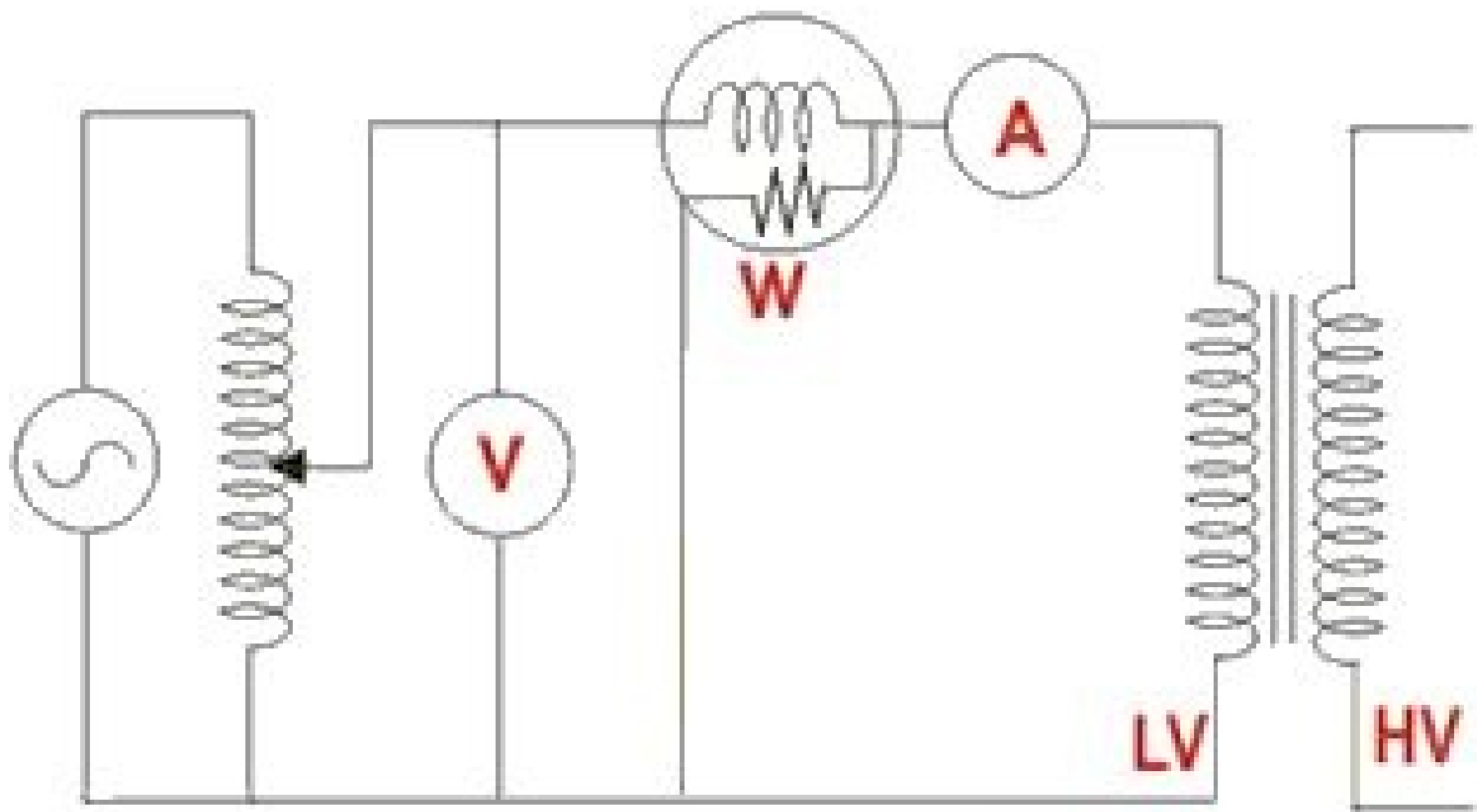
Open Circuit Test on Transformer
